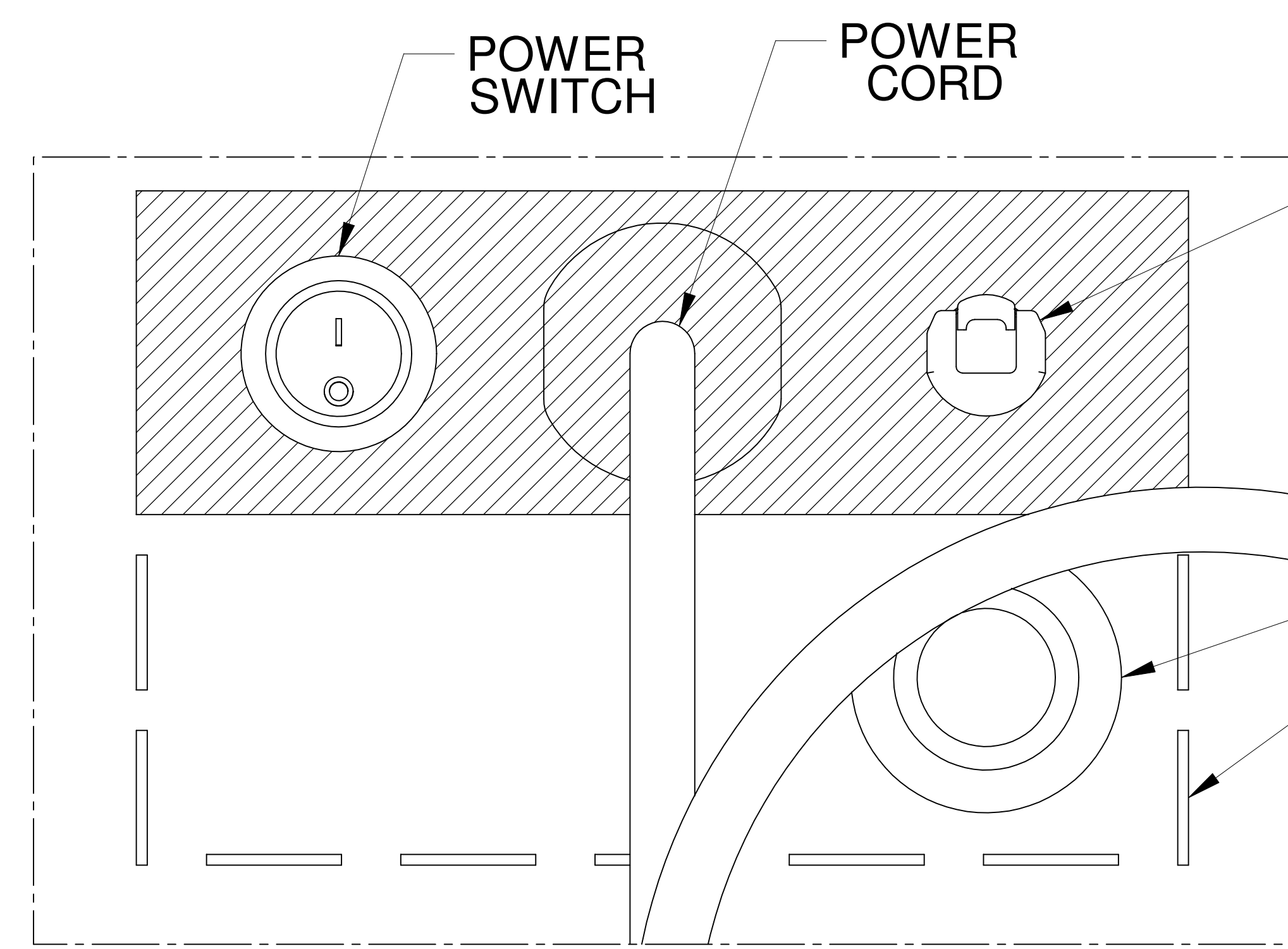
DETAIL A
