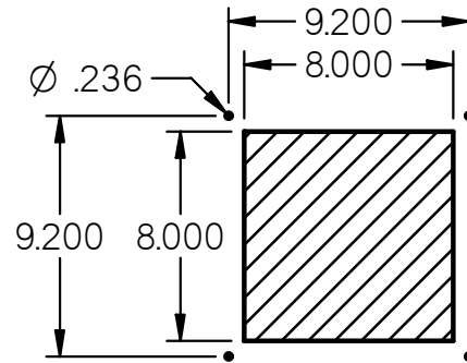
200 MFFPCUTOUT DRAWING 1:8
